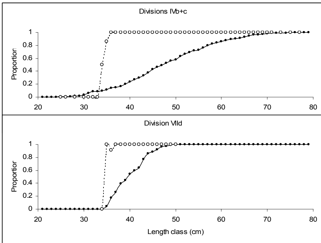
Figure 6. The cumulative proportion of bass at each length class in the total catch (solid line) and the proportion retained (dotted line, open circle) by trawlers using 90 mm mesh nets.
