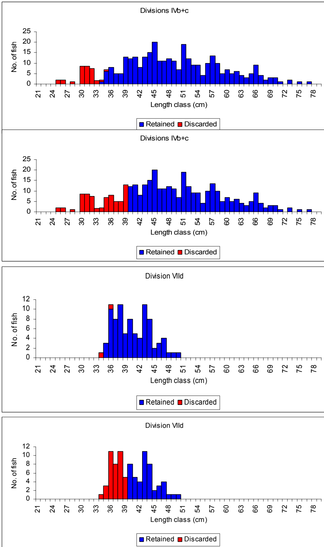
Figure 10. Pairs of length distributions showing the current patterns of retention/discarding and the effect that a 40 cm MLS may have on catches, for bass caught in 100 mm mesh trawls.
